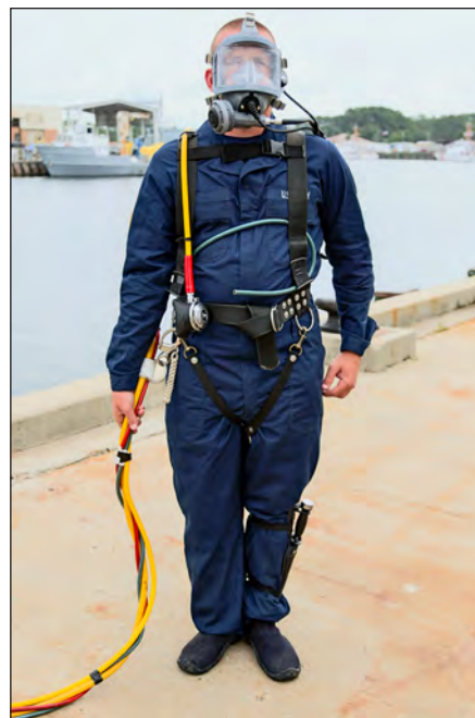
Figure 8-6. MK 20 MOD 0 UBA.
