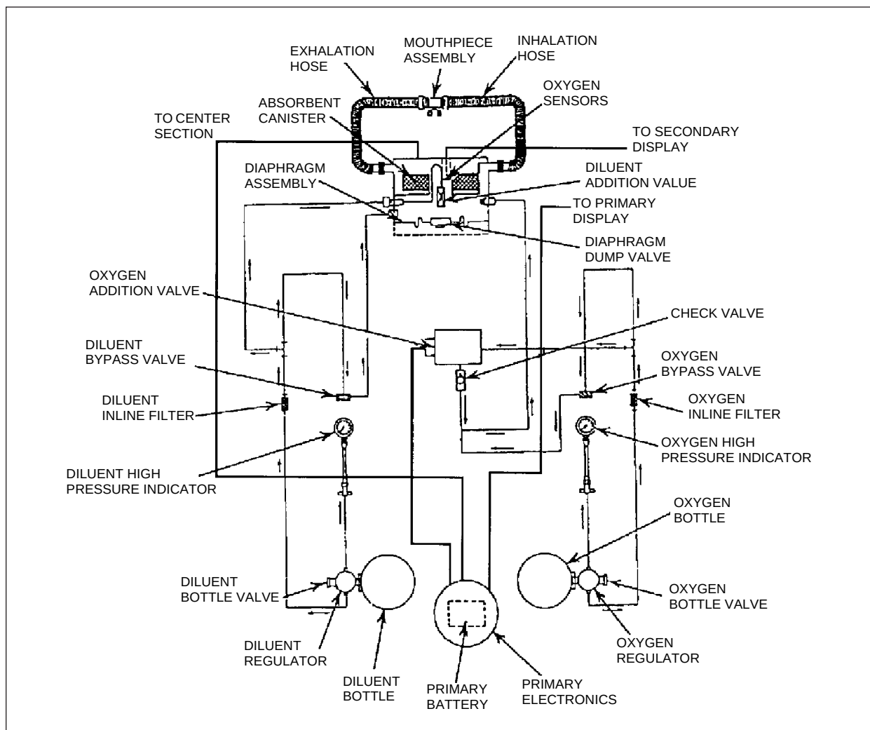
Figure 15-2. Typical EC-UBA Functional Diagram.
